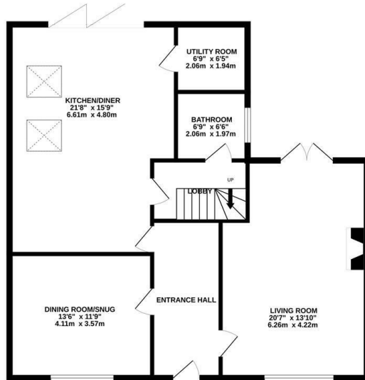
GROUND FLOOR 977 sq.ft. (90.8 sq.m.) approx.
